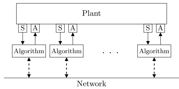
Fig. 2. The considered networked control architecture: the blocks A and S denote (possibly heterogeneous) actuator and sensor units; the Algorithm block includes estimation and control algorithms as well as the communication logic.
